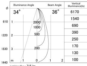
■ Direct Horizontal Illuminance DD133-0835W9030
