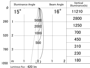
■ Direct Horizontal Illuminance DD133-0515W9030
