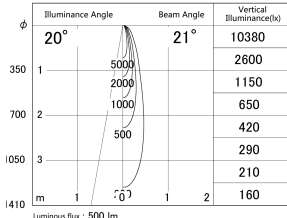
■ Direct Horizontal Illuminance DD133-0520W9030
