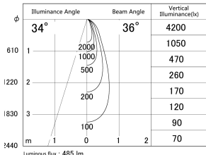
■ Direct Horizontal Illuminance DD133-0535W9030
