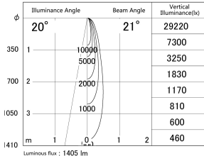
■ Direct Horizontal Illuminance DD133-1420W9035
