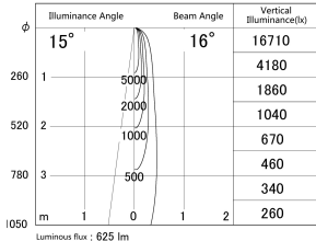
■ Direct Horizontal Illuminance DD133-0815W9035
