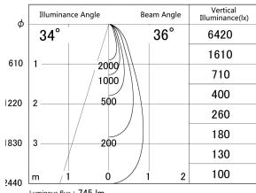
■ Direct Horizontal Illuminance DD133-0835W9035
