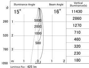
■ Direct Horizontal Illuminance DD133-0515W9035
