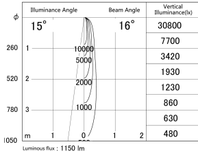
■ Direct Horizontal Illuminance DD133-1415W9040
