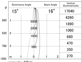
■ Direct Horizontal Illuminance DD133-0815W9040
