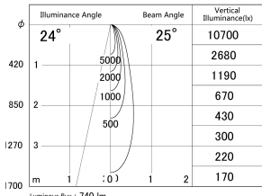
■ Direct Horizontal Illuminance DD133-0825W9040
