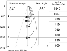
■ Direct Horizontal Illuminance DD133-0835W9040
