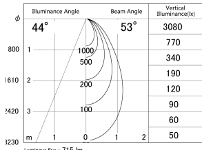
■ Direct Horizontal Illuminance DD133-0850W9040
