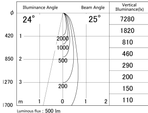
■ Direct Horizontal Illuminance DD133-0525W9040
