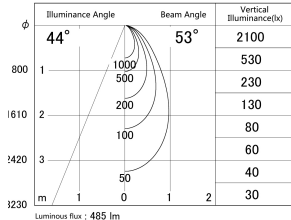
■ Direct Horizontal Illuminance DD133-0550W9040
