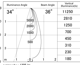
■ Direct Horizontal Illuminance DD133-1435B9027
