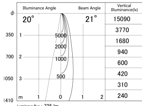
■ Direct Horizontal Illuminance DD133-0820B9027
