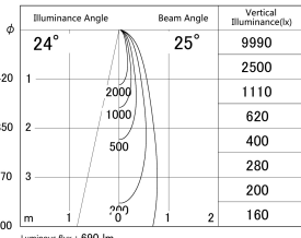
■ Direct Horizontal Illuminance DD133-0825B9027
