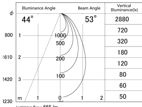
■ Direct Horizontal Illuminance DD133-0850B9027
