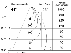
■ Direct Horizontal Illuminance DD133-0550B9027
