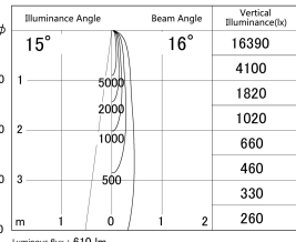
■ Direct Horizontal Illuminance DD133-0815B9030
