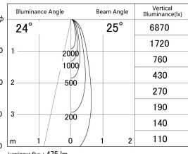
■ Direct Horizontal Illuminance DD133-0525B9030
