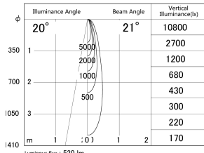
■ Direct Horizontal Illuminance DD133-0520B9035
