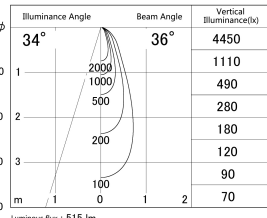
■ Direct Horizontal Illuminance DD133-0535B9040
