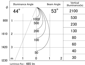
■ Direct Horizontal Illuminance DD133-0550B9040
