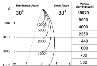
■ Direct Horizontal Illuminance DD126-4035W9030-LX
