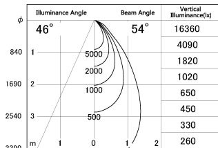
■ Direct Horizontal Illuminance DD126-3755W9030-LX
