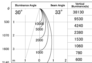
■ Direct Horizontal Illuminance DD126-4035W9040-LX
