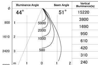
■ Direct Horizontal Illuminance DD126-3755MW9027-LX
