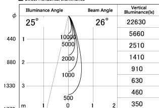
■ Direct Horizontal Illuminance DD126-1425MW9027-LX
