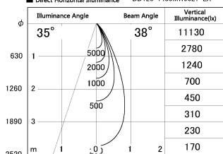
■ Direct Horizontal Illuminance DD126-1435MW9027-LX
