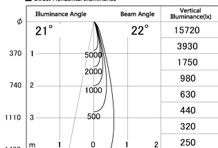
■ Direct Horizontal Illuminance DD126-0825MW9027-LX
