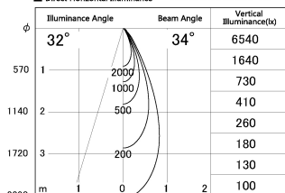
■ Direct Horizontal Illuminance DD126-0835MW9027-LX
