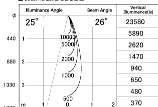
■ Direct Horizontal Illuminance DD126-1425MW9030-LX
