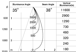
■ Direct Horizontal Illuminance DD126-1435MW9030-LX
