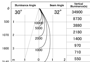
■ Direct Horizontal Illuminance DD126-3735MW9035-LX
