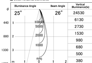
■ Direct Horizontal Illuminance DD126-1425MW9035-LX
