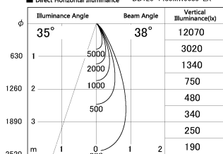
Direct Horizontal Illuminance DD126-1435MW9035-LX
