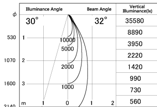
■ Direct Horizontal Illuminance DD126-3735MW9040-LX
