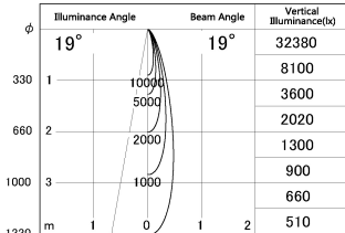
■ Direct Horizontal Illuminance DD126-1415MW9040-LX
