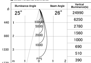
■ Direct Horizontal Illuminance DD126-1425MW9040-LX
