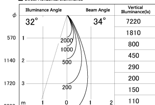
■ Direct Horizontal Illuminance DD126-0835MW9040-LX
