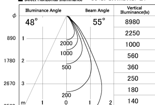
■ Direct Horizontal Illuminance DD126-2555MB9027-LX
