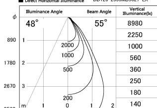
■ Direct Horizontal Illuminance DD126-2555MB9027-LX
