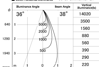
■ Direct Horizontal Illuminance DD126-2035MB9027-LX
