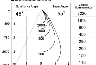
■ Direct Horizontal Illuminance DD126-2055MB9027-LX
