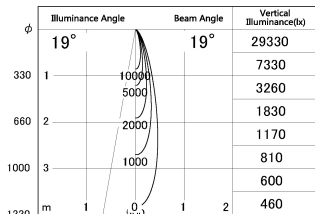
■ Direct Horizontal Illuminance DD126-1415MB9027-LX
