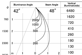
■ Direct Horizontal Illuminance DD126-1455MB9027-LX
