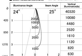
■ Direct Horizontal Illuminance DD126-2525MB9030-LX
