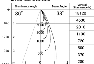
■ Direct Horizontal Illuminance DD126-2535MB9030-LX
