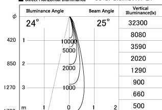
■ Direct Horizontal Illuminance DD126-2025MB9030-LX
